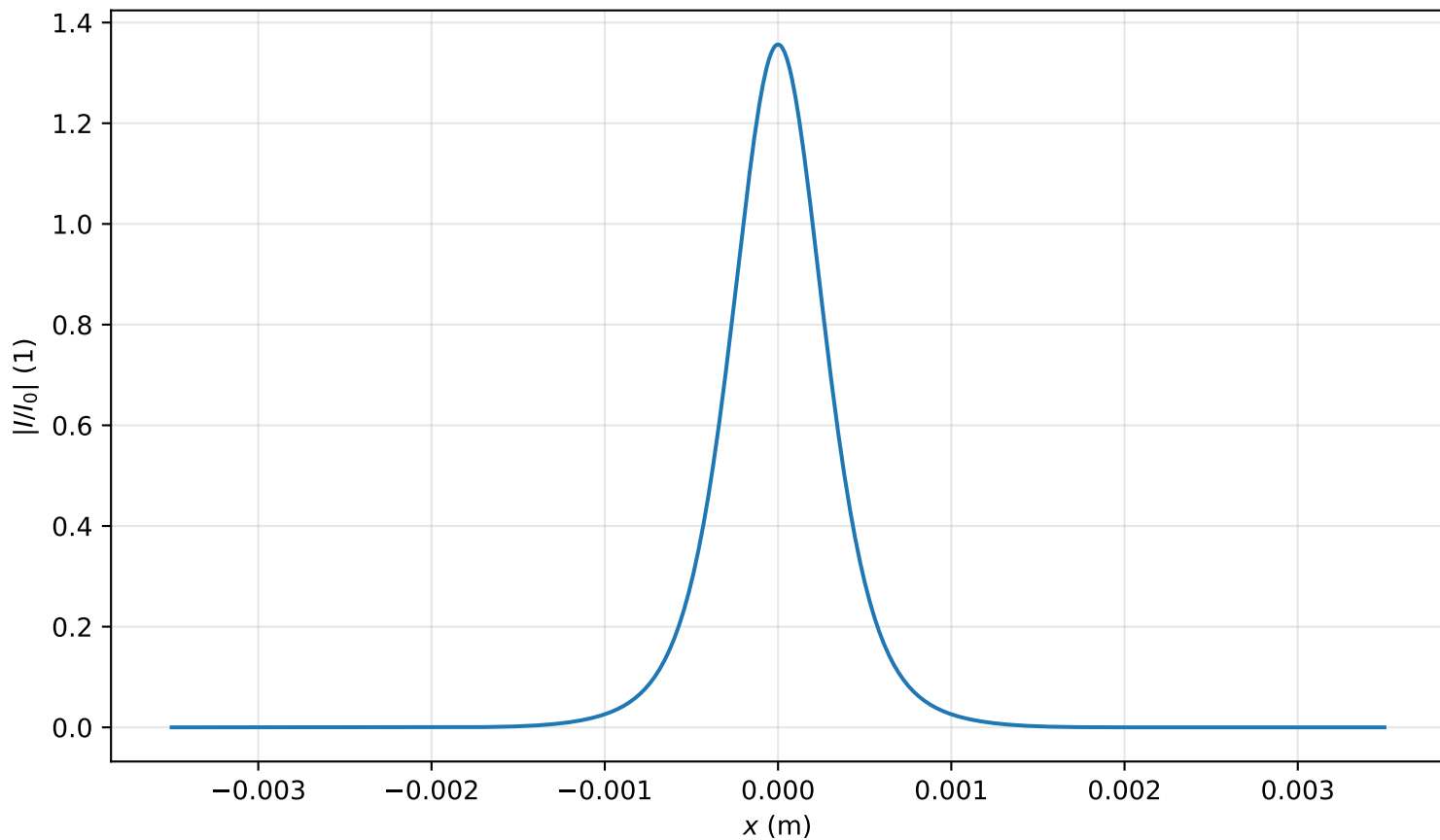
Intensity profile I(x, y = 0, z = 1.592m)/I_0 , P_{in}=0.8P_{cr} , artificial time
